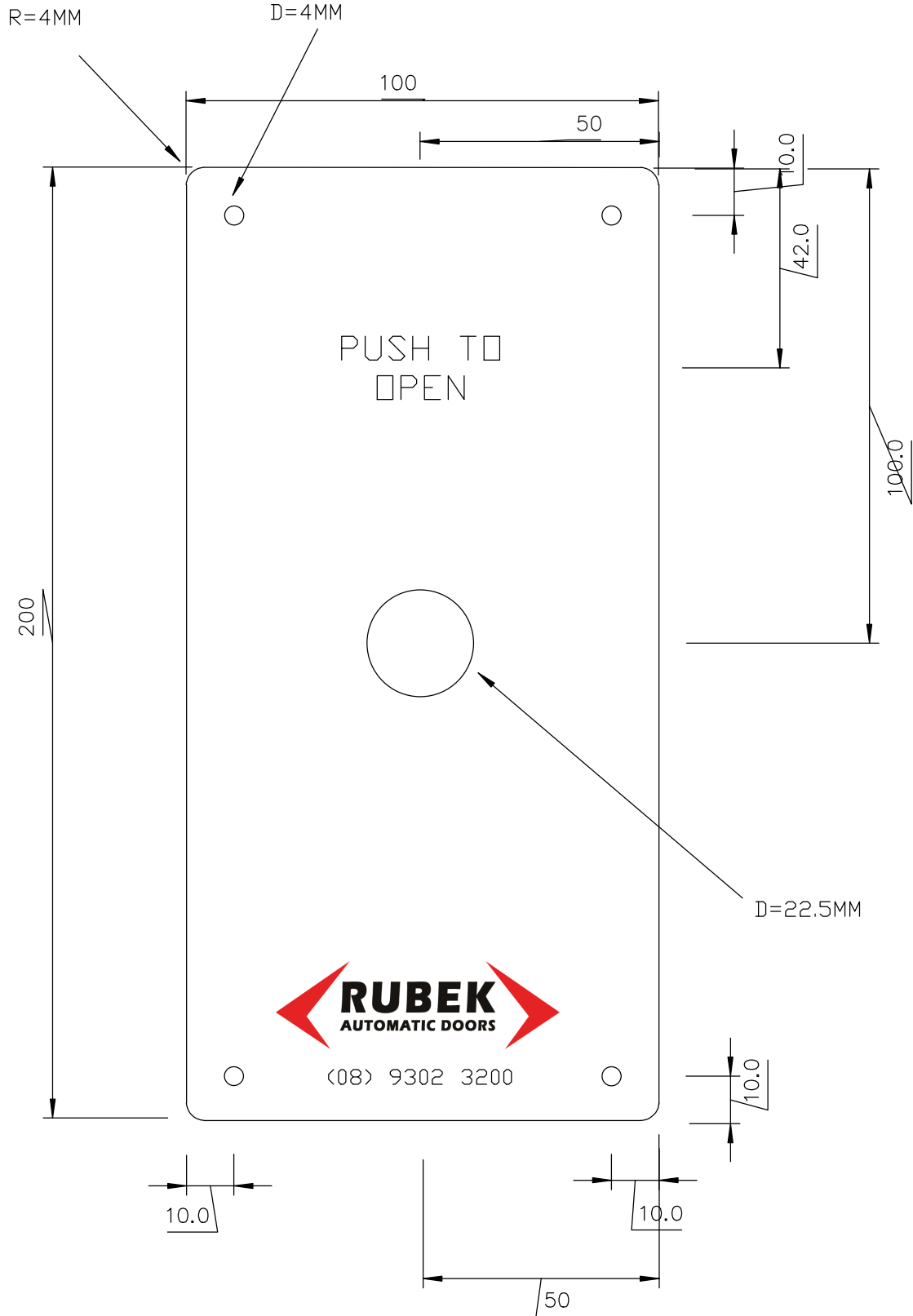
FRONT VIEW OF OUTSIDE DOOR CONTROL
