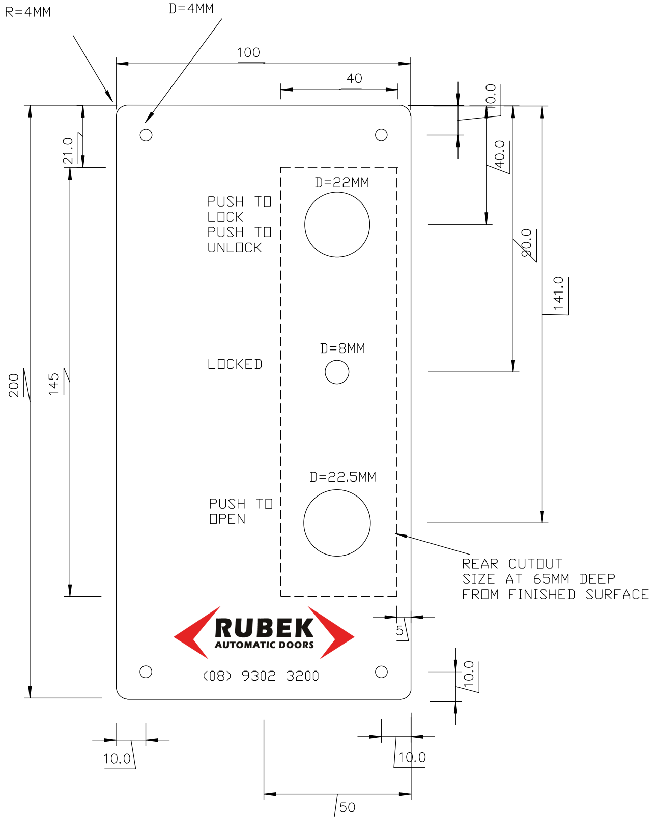
FRONT VIEW OF INSIDE DOOR CONTROL
