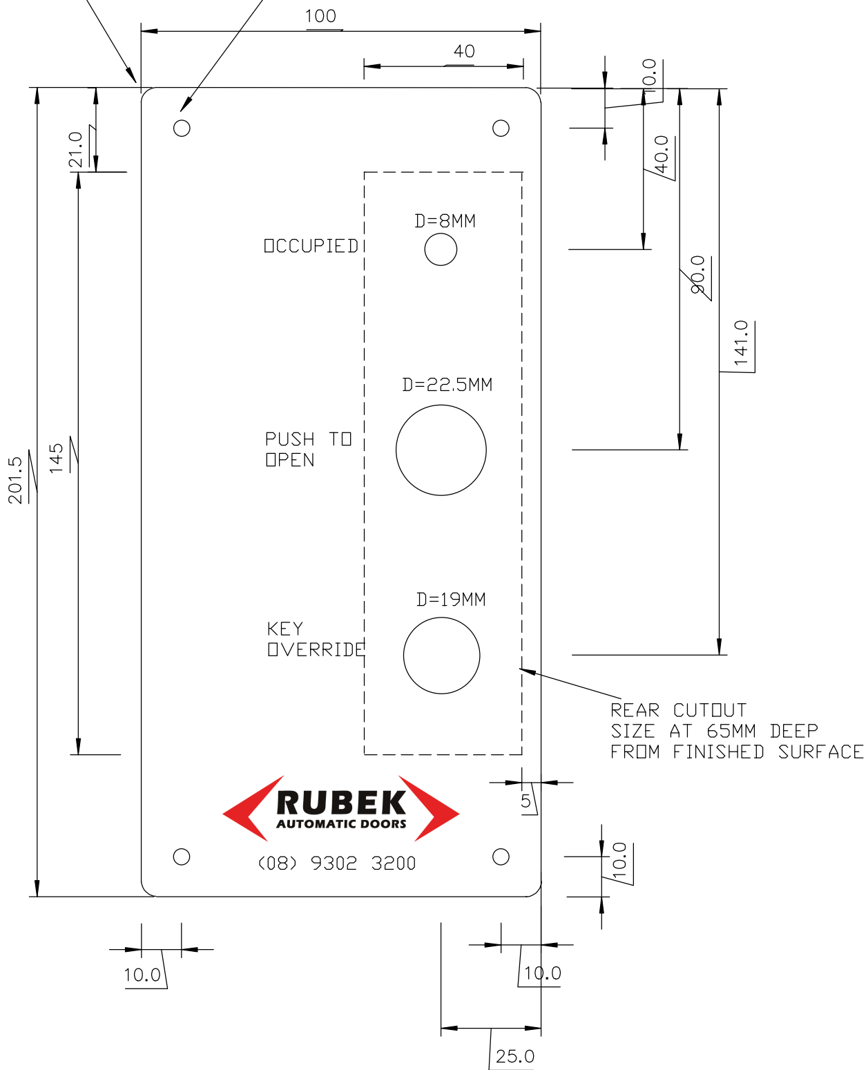
FRONT VIEW OF OUTSIDE DOOR CONTROL
