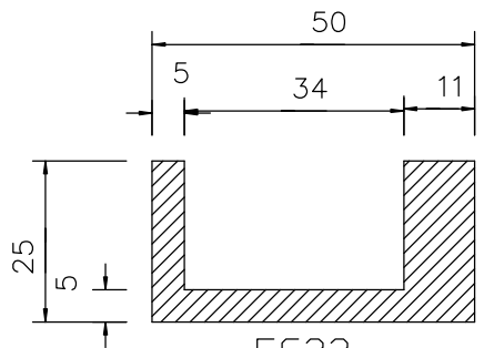
FG32 TO SUIT DORMA BOTTOM RAIL WHITE NYLON
