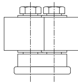
FG1 TO SUIT ALUMINIUM FRAMED DOORS
